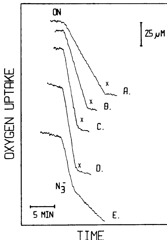
Fig.1. Oxygen uptake of air-saturated solutions containing HPD ( \sim 1:100 dilution of Photofrin II, absorbance = 2 for a 1 cm path at 365 nm) and cysteine in pH 7.8 phosphate buffer. Irradiation with filtered white light was initiated at 'ON' for each solution. For solutions A-D the light was turned off at 'x' and 1000 units/ml of catalase was added. Cysteine concentrations were: (A) 1 mM, (B) 5 mM, (C) 10 mM, (D) 25 mM, and (E) 5 mM. Azide at a final concentration of 5 mM was added at the break in curve E as irradiation continued. No rapid uptake of oxygen was observed in an irradiated HPD solution in the absence of cysteine (not shown).
